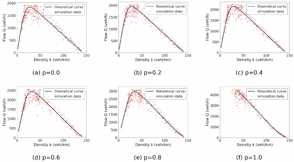
Figure 2. Comparison between simulation results and analytical FD model
